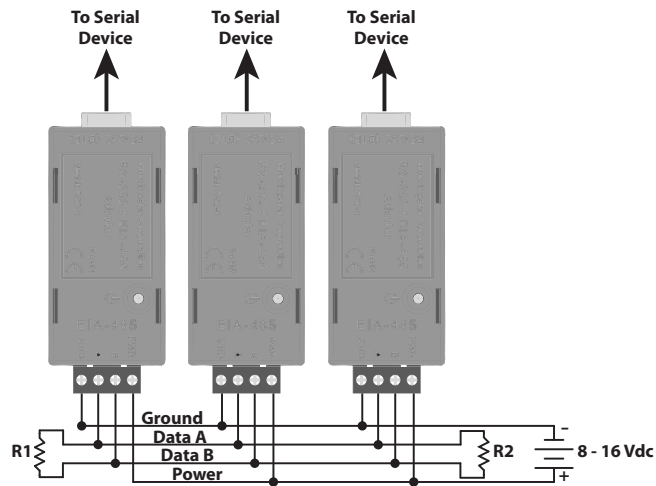
Figure 4. EIA-485 bus wiring
